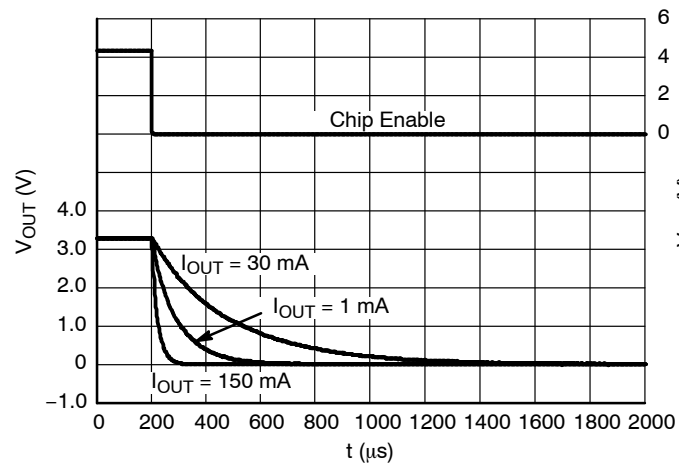
Figure 37. Shutdown, 3.3 V Version D, V_{\text{IN}} = 4.3 \text{ V}
