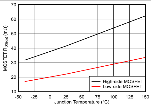
Figure 6-6. High-Side and Low-Side MOSFET R_{DS(on)}
