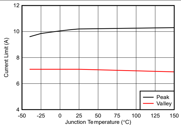
Figure 6-4. High-Side and Low-Side Current Limits
