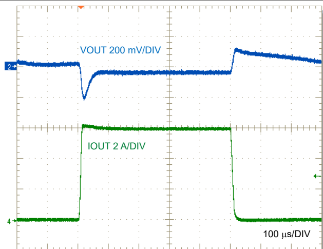
Figure 8-27. LM634x0-Q1 Load Transient, I_{OUT} = 0A to 6A
