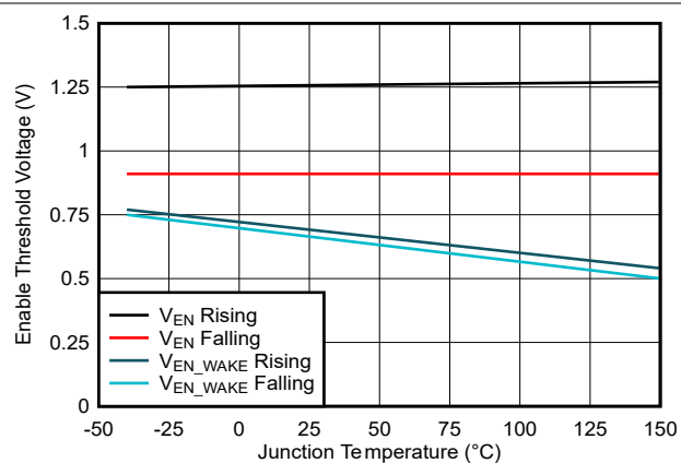
Figure 6-7. Enable Thresholds
