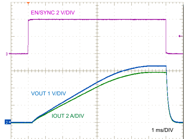
Figure 8-25. LM634x0-Q1 Enable On, Off, 6A Resistive Load
