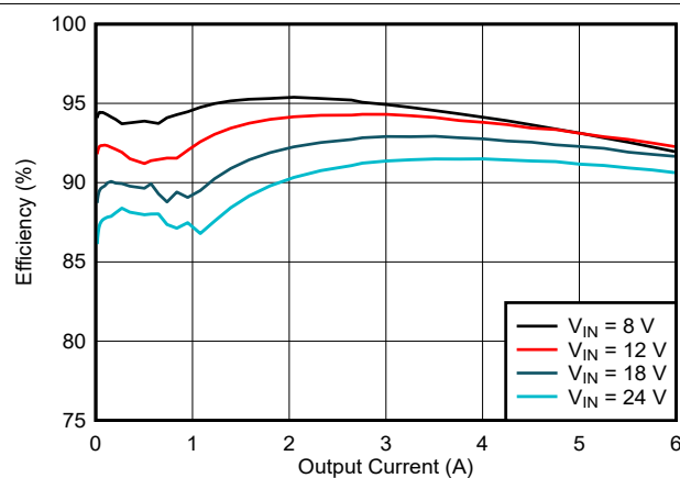
Figure 8-3. LM634x0-Q1 Efficiency
