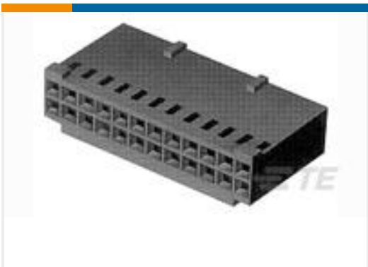
TE Part #280365 AMPMODU, DBL ROW, CONTACT REC
