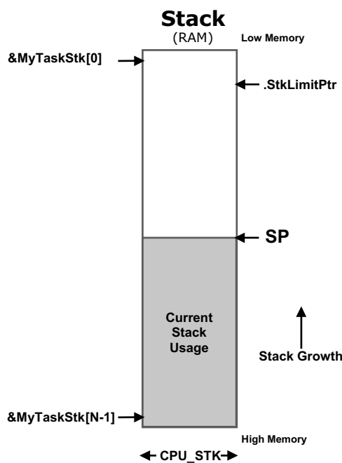
Figure 5-3 Hardware detection of stack overflows
