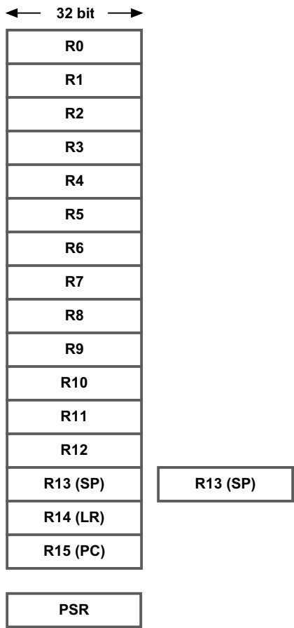
Figure 2-1 The Cortex-M3 CPU Registers
