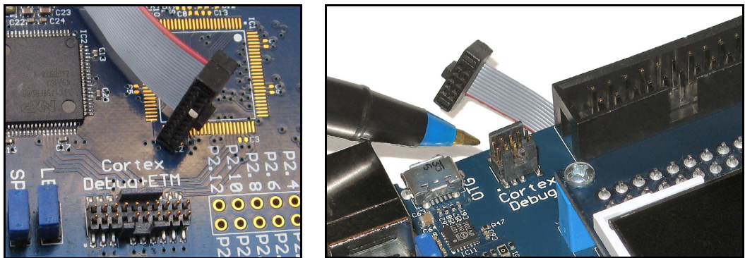
Figure D-6 20 pin ETM and 10 pin Hi-density JTAG/SWD
