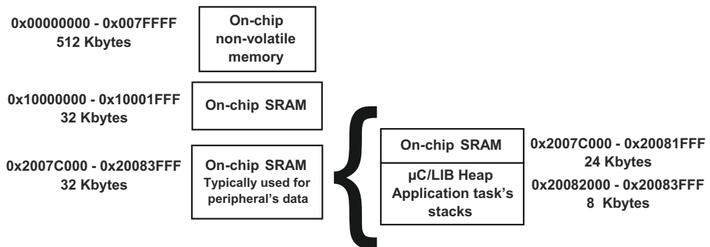
Figure 4-11 Memory Layout
