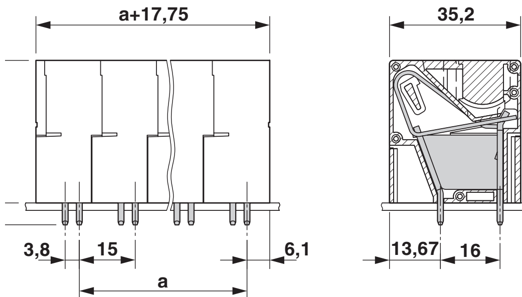
Dimensional drawing
