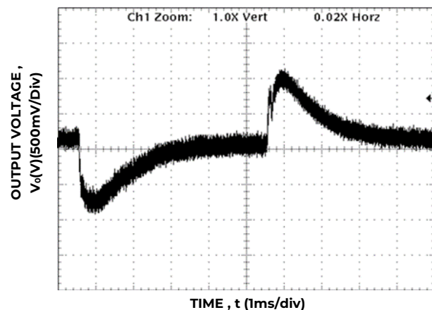
Figure 7. 12V Transient response load step 20–120A, V_{IN} = -48V_{DC}
