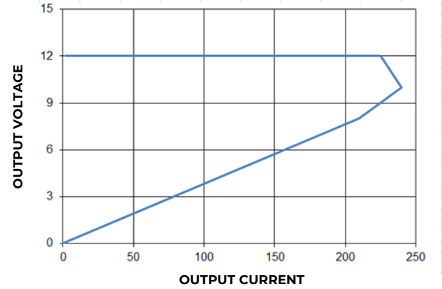
Figure 2. 12V output : Current limit profile ( V_{in} : -48V_{DC} )
