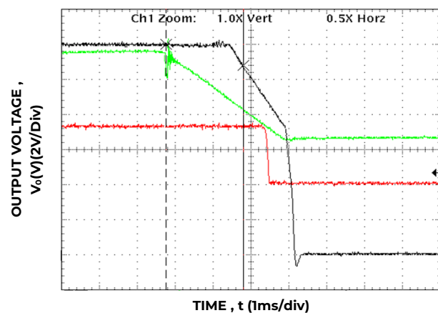
Figure 9. 12V holdup time, full load, V_{IN} = -48V_{DC}
