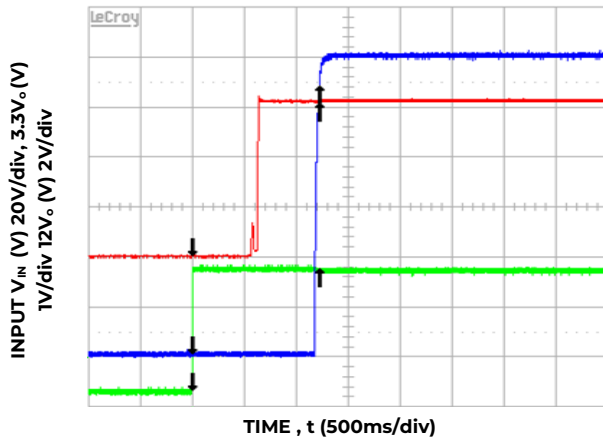
Figure 3. Input start up ( V_{in} = -48V_{DC} , full load ).
