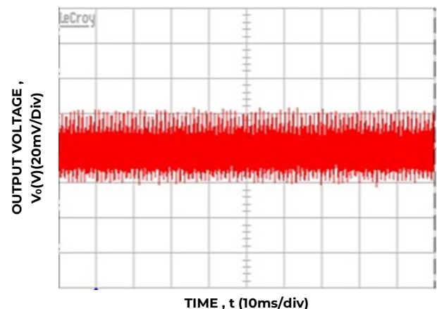
Figure 6. 3.3V output ripple and noise ( V_{in} : -48V_{dc} , full load)
