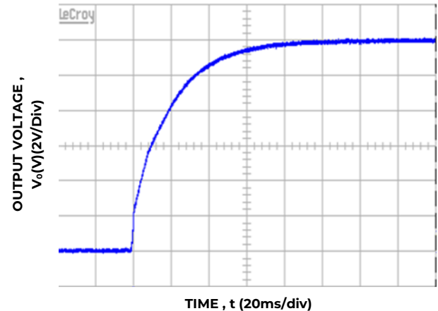
Figure 4. 12V start-up ( V_{in} : -48V_{DC} , full load)
