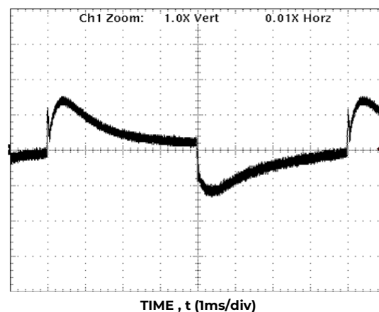
Figure 8. 12V Transient response 100 – 200A, V_{IN} = -48V_{DC}
