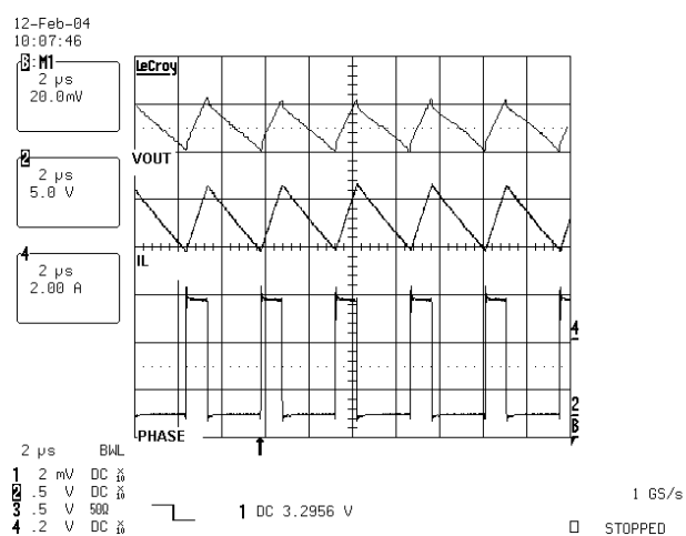
FIGURE 5. PWM WAVEFORMS
