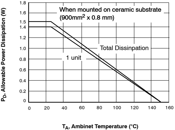
Figure 12. P_D - T_A
