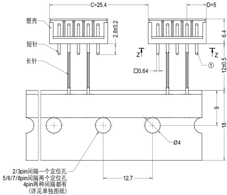
EH-5A(2.4长针)编带装
