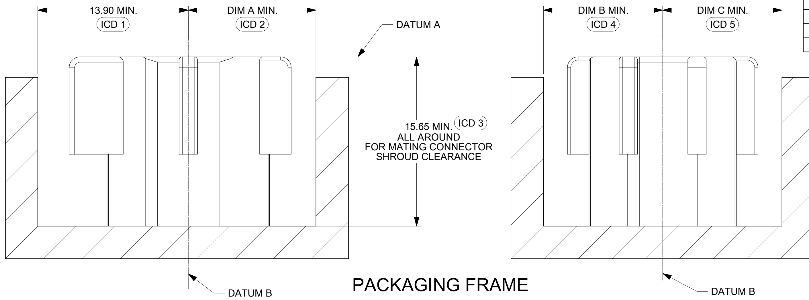
PACKAGING FRAME
