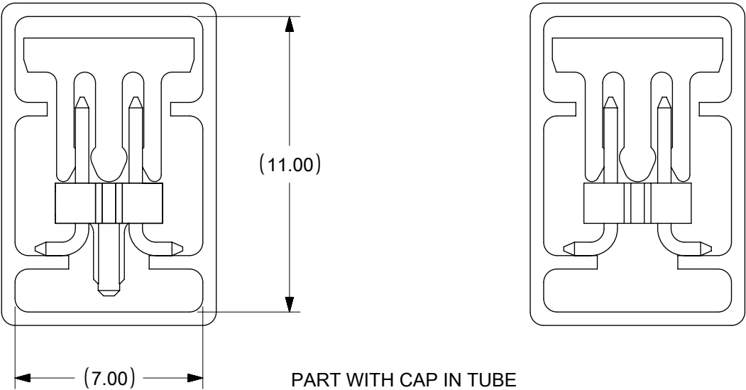
PART WITH CAP IN TUBE (PLS REFER TO PK SPEC: PK-89990-476)
