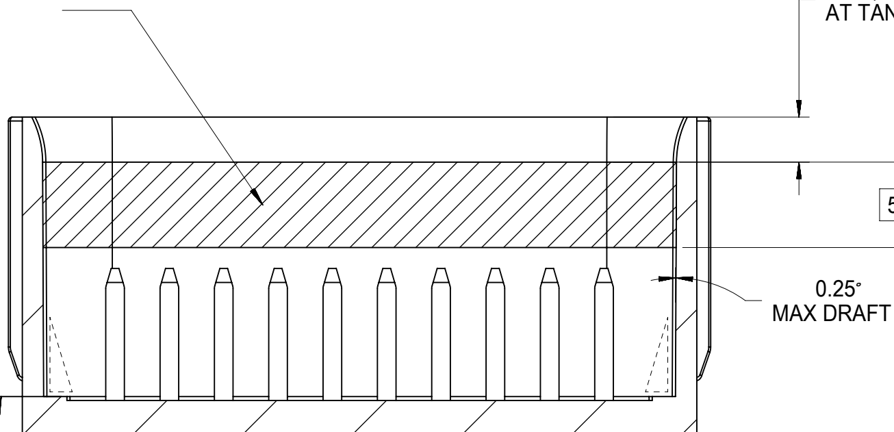
SECTION B-B
