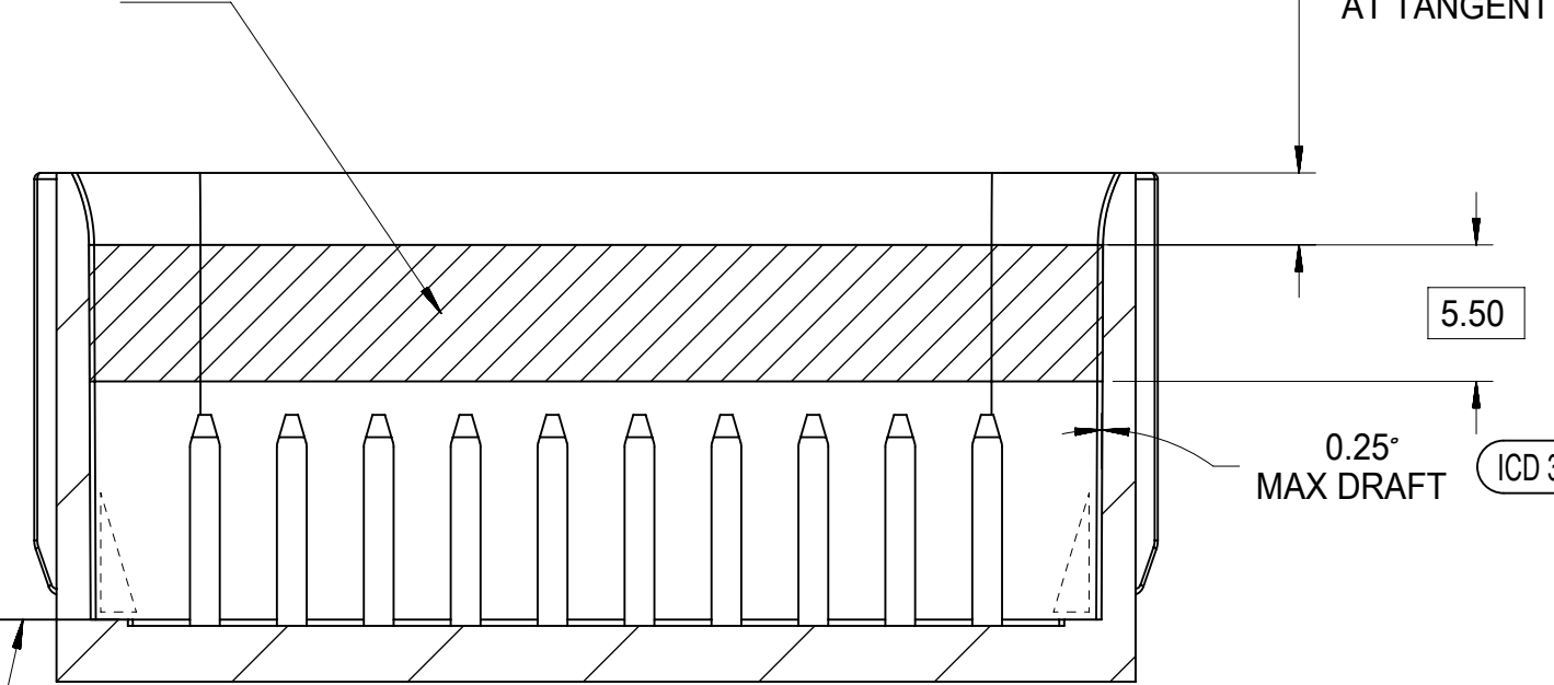
SECTION B-B
