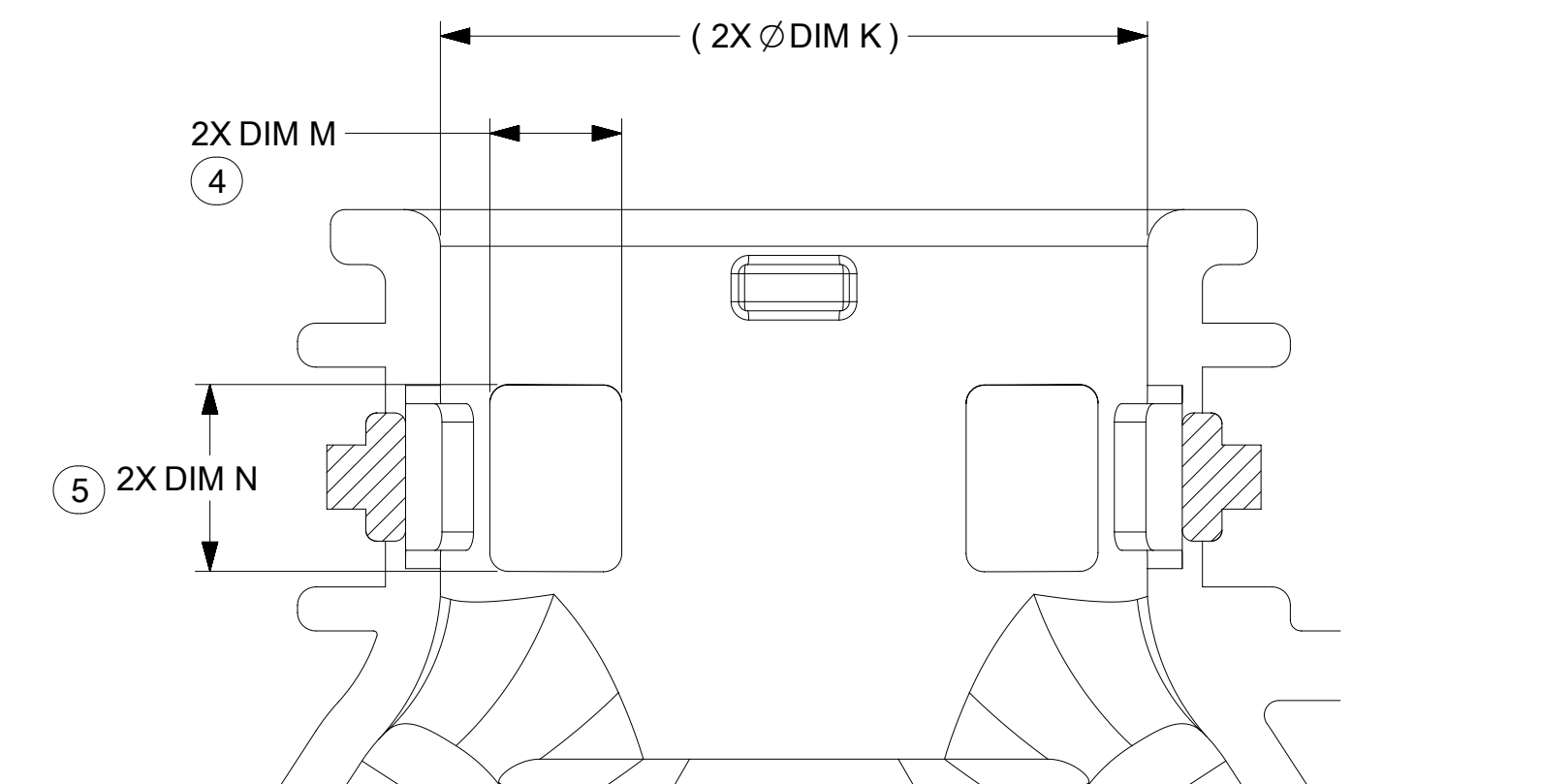
PARTIAL SECTION D-D SCALE 5:1 WITHOUT RIBS
