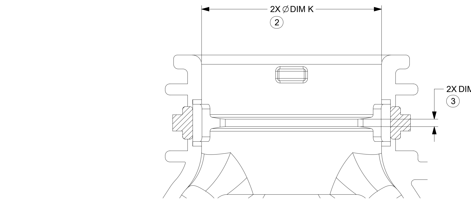
PARTIAL SECTION C-C SCALE 5:1 WITH RIBS
