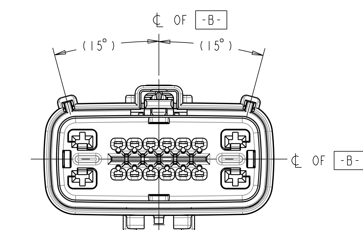
KEYING OPTION D SCALE 2:1
