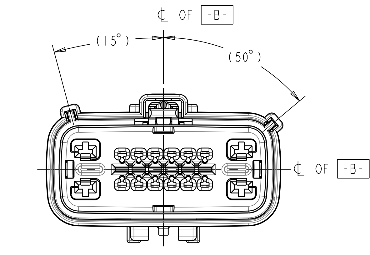
KEYING OPTION C SCALE 2:1
