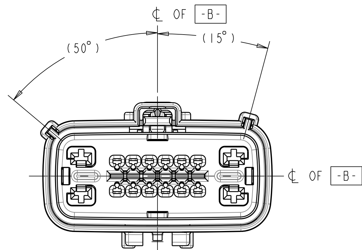
KEYING OPTION B SCALE 2:1
