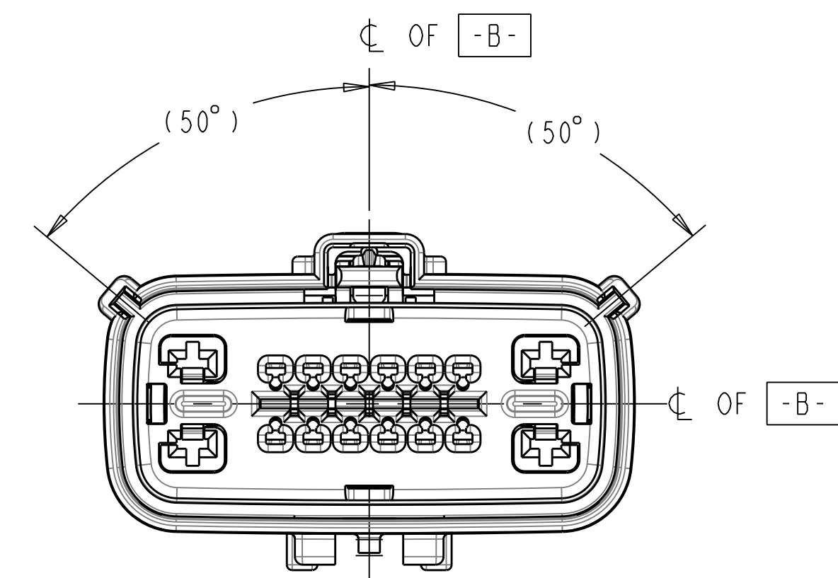
KEYING OPTION A SCALE 2:1
