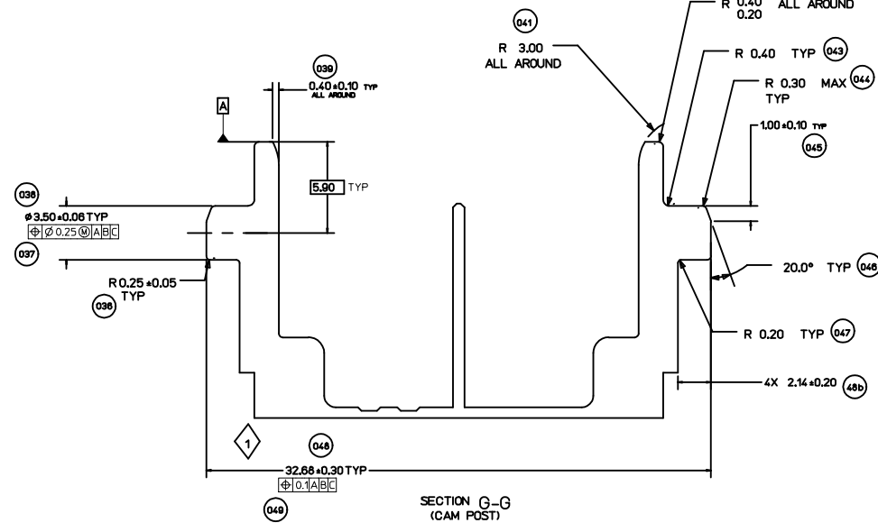
VIEW YY TYPICAL
