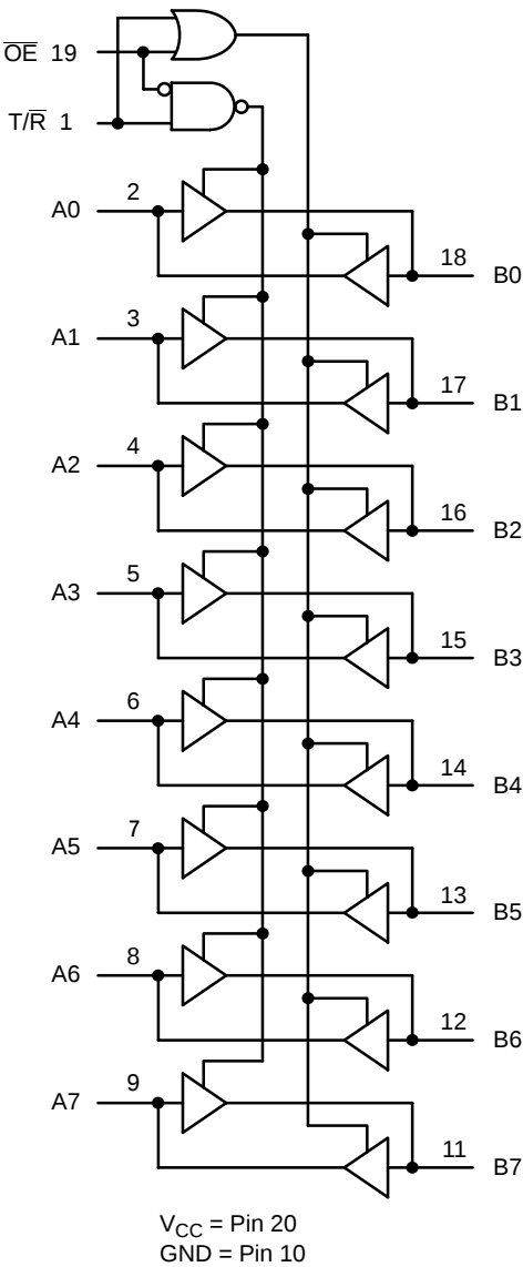
Figure 1. Logic Diagram
