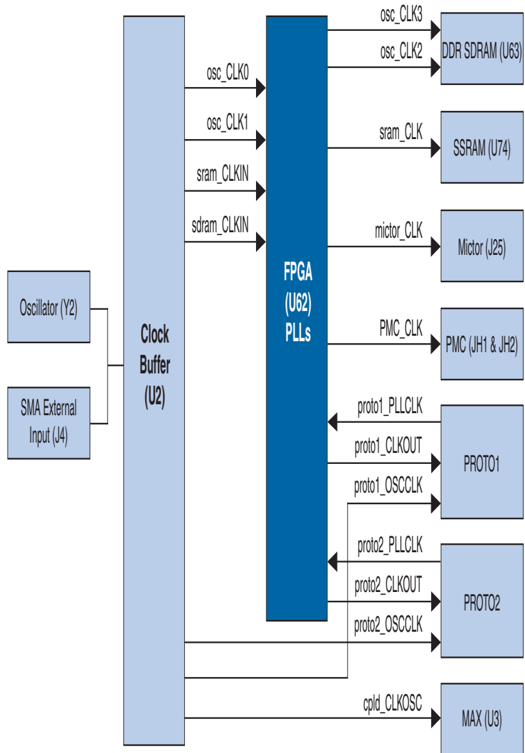
Figure 2–21. Clock Circuitry
