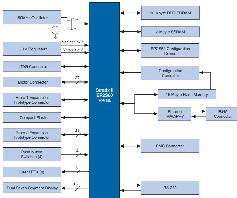
Figure 1–1. Nios Development Board, Stratix II Edition Block Diagram
