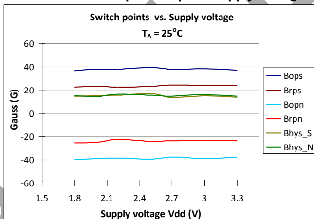
Switch Points Bop and Brp vs. Supply Toltage
