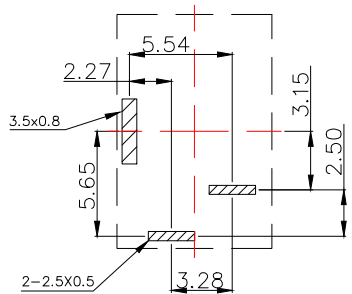
PCB.WELDING DRAWING (TOLERANCE: ±0.05)
