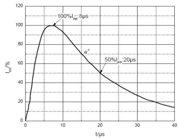
8/20 \mu s pulse waveform according to IEC 61000-4-5
