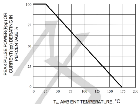
Fig. 2-PULSE RATING CURVE
