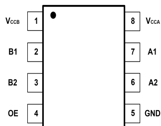
RS0102YH8 (SOT-23-8L) Package
