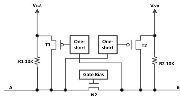
Architecture of RS0102YH8
