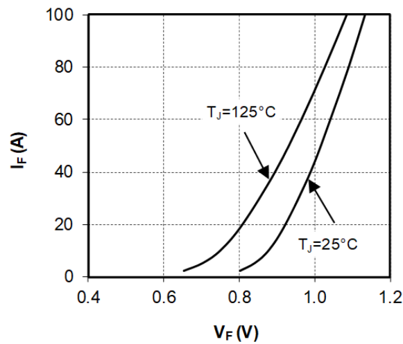
Figure 1-2. Forward Characteristics
