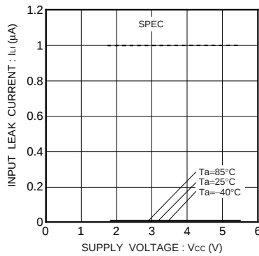
Fig.21 Input leakage current I_{II} (A1,A2,SCL,WP)
