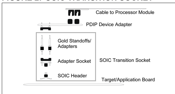
FIGURE 2: SOIC TRANSITION SOCKET
