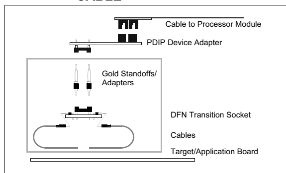
FIGURE 10: DFN TRANSITION SOCKET WITH CABLE
