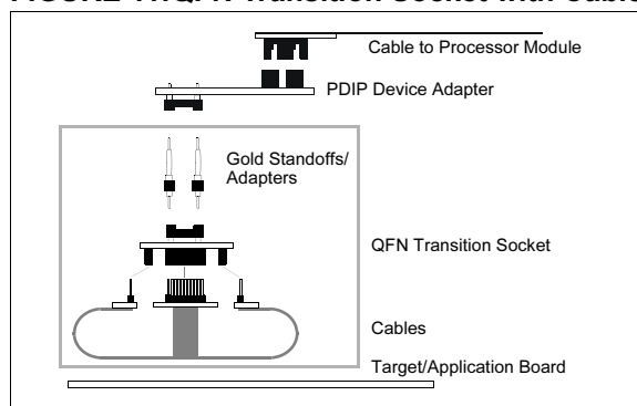
FIGURE 11: QFN Transition Socket with Cable
