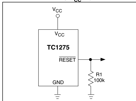
FIGURE 3-6: ENSURING \overline{\text{RESET}} VALID TO V_{CC} = 0V
