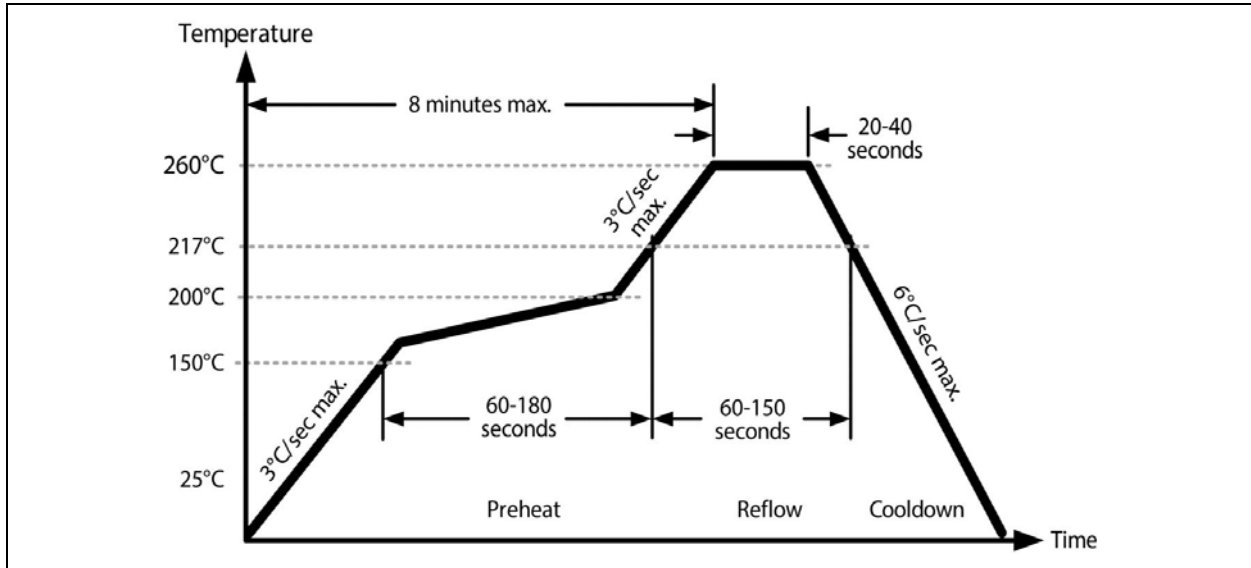
MSL 1 @ 260°C refer to JSTD-020C
