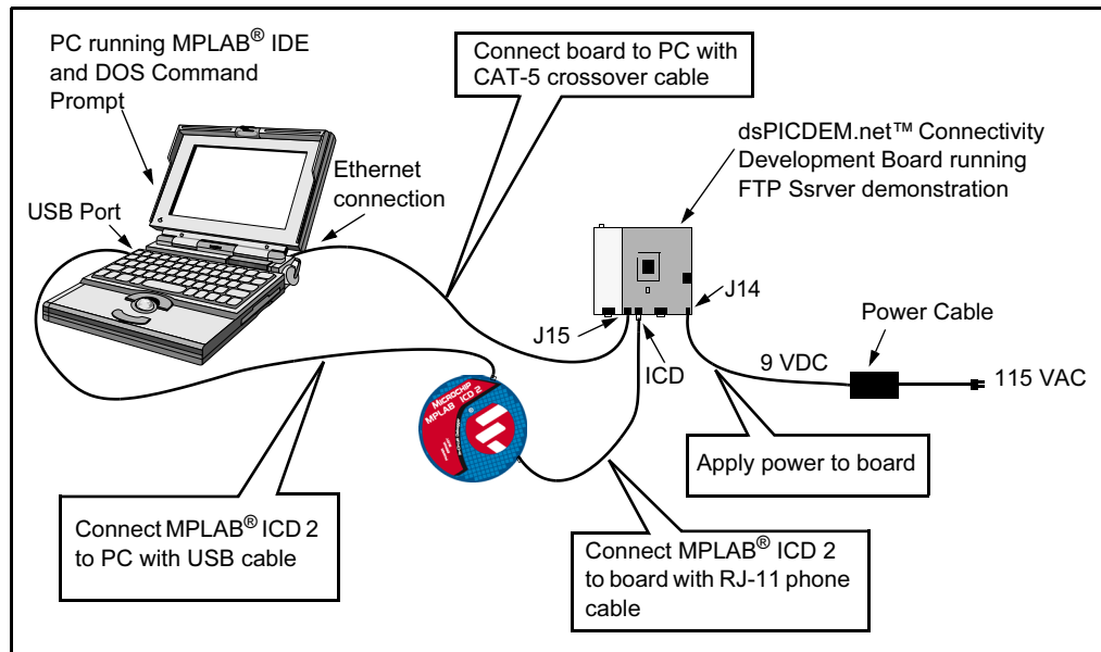
FIGURE 5-1: FTP SERVER DEMONSTRATION SETUP
