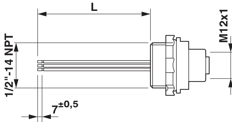
Dimensional drawing
