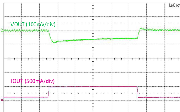
Figure 18. Load Transient, I_{OUT} = 100 \leftrightarrow 500\text{ mA} , 1\text{ }\mu\text{s} Edge, V_{OUT} = 3.15\text{ V}
