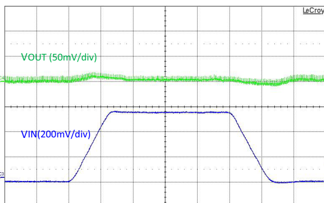
Figure 20. Line Transient, V_{IN} = 2.5\text{ V} \leftrightarrow 3.0\text{ V} , 10\text{ }\mu\text{s} Edge, I_{OUT} = 300\text{ mA}
