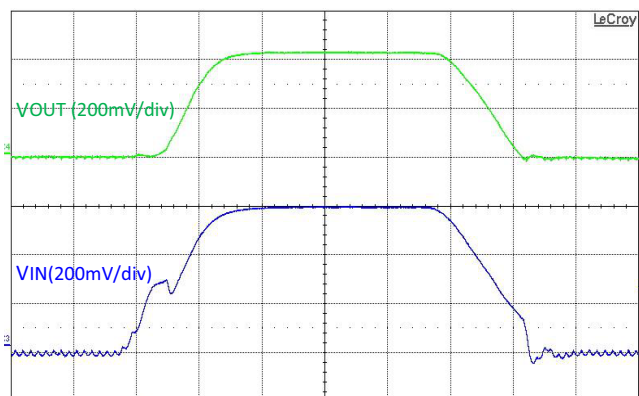
Figure 19. Line Transient, V_{IN} = 3.0\text{ V} \leftrightarrow 3.6\text{ V} , 10\text{ }\mu\text{s} Edge, I_{OUT} = 500\text{ mA} , V_{OUT} = 3.15\text{ V}
