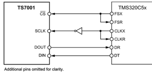
Figure 15: Interfacing the TS7001 to TMS320C5x-type DSPs.
