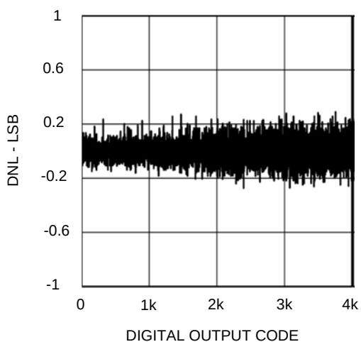
Differential Nonlinearity
