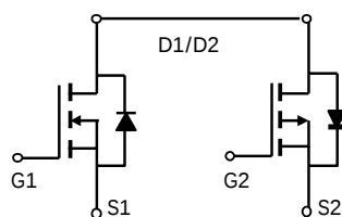
N-channel
