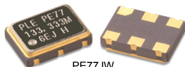
PE77JW 5.0 x 7.0 x 1.70 mm LCC Ceramic Package
