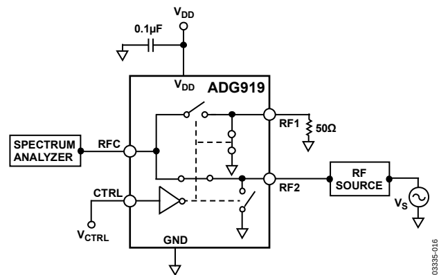
Figure 25. P_{-1\text{ dB}}
