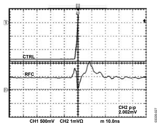
Figure 15. Video Feedthrough
