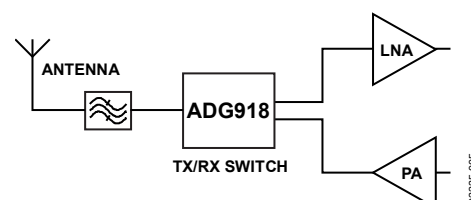
Figure 26. Wireless Metering
