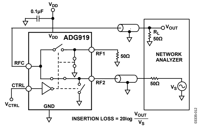
Figure 21. Insertion Loss
