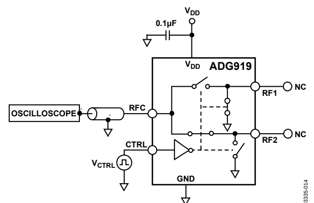
Figure 23. Video Feedthrough
