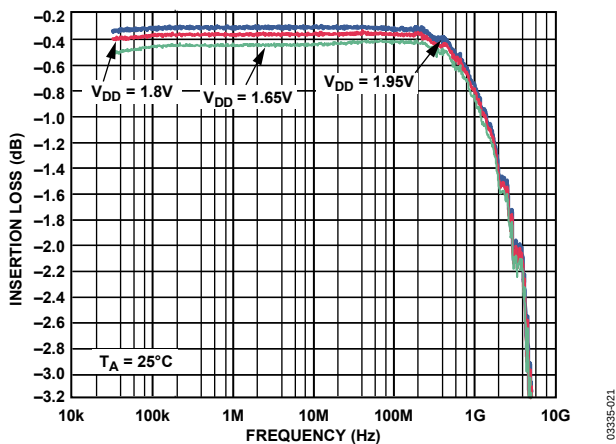
Figure 7. Insertion Loss vs. Frequency over Supplies (RF1/RF2, S12, and S21)
