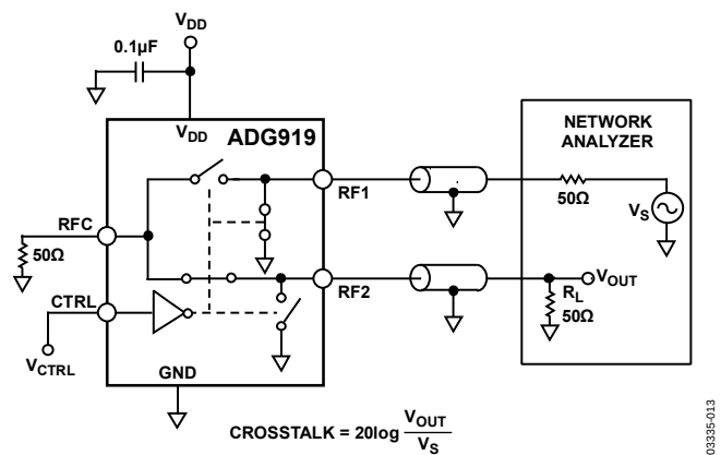
Figure 22. Crosstalk
