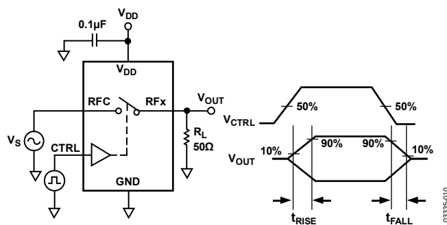
Figure 19. Switch
