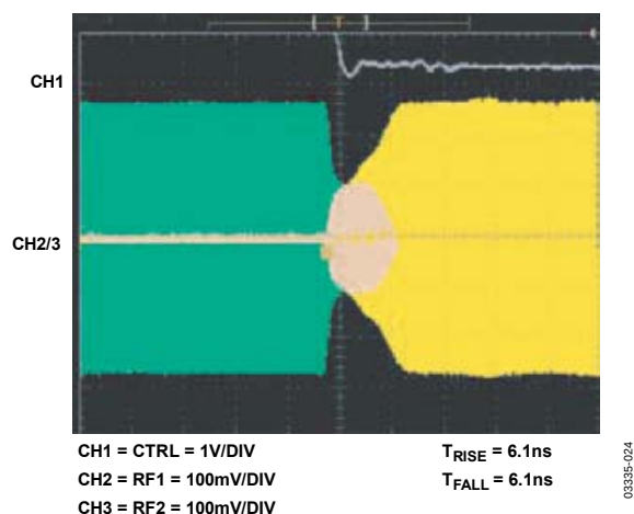
Figure 14. Switch Timing
