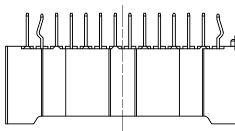
11~15極形状（反ロック面） FIGURE OF 11-15 CIRCUIT (UN-LOCK SIDE)
