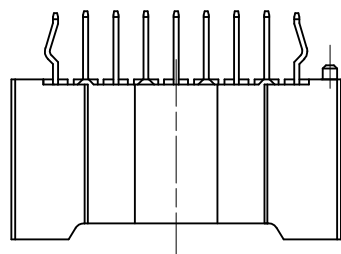
8~10 極形状 (反ロック面) FIGURE OF 8-10 CIRCUIT (UN-LOCK SIDE)
