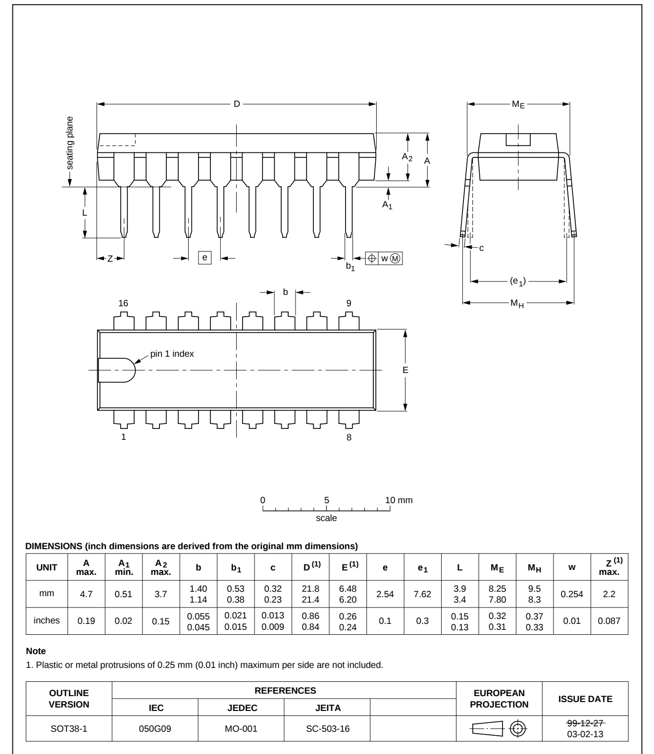
Fig 11. Package outline SOT38-1 (DIP16)
