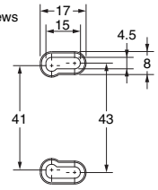
Mounting Holes (Enlargement)
