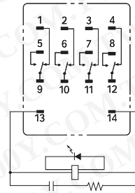
MY4NJ-CR
