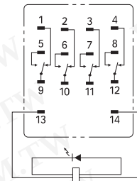
MY4NJ-CR
