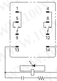
MY2NJ-CR
