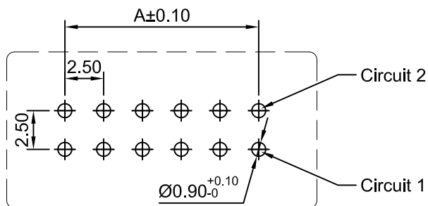
P.C.B LAYOUT (TOP VIEW) TOLERANCE:±0.05
