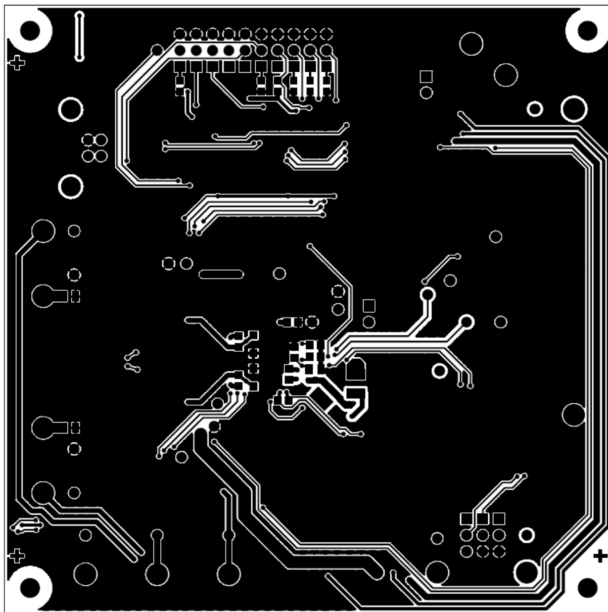
Figure 13. Layer2 Routing
