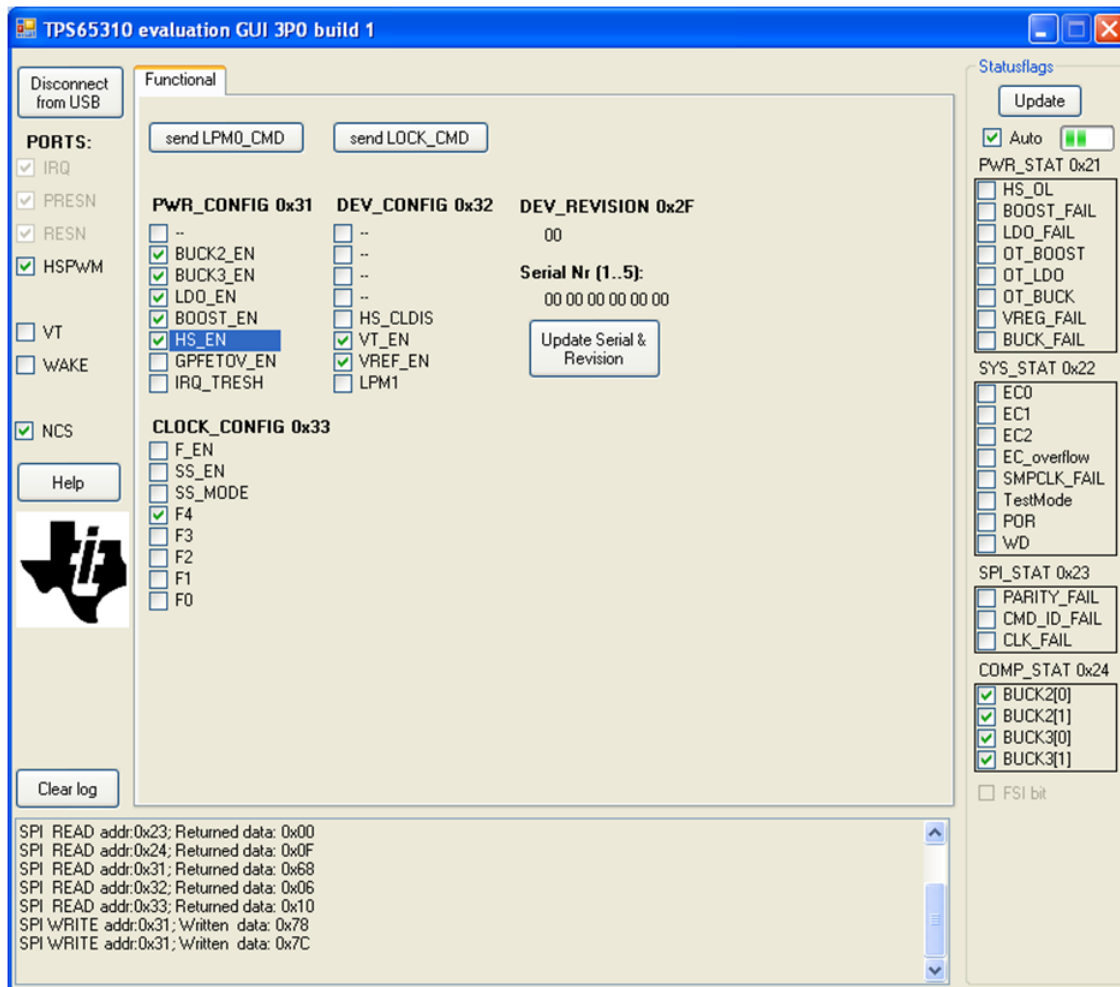
Figure 5. GUI Software HS EN ON and HS PWM ON
