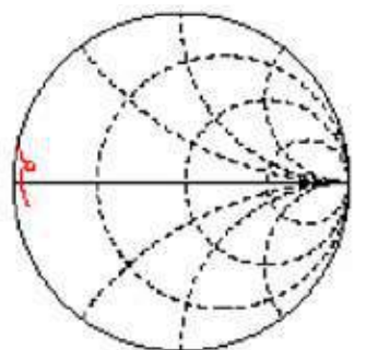
Typical S11 Frequency Range: 1.0 to 20 GHz Reflection Coefficient: 50 \Omega Normalized
