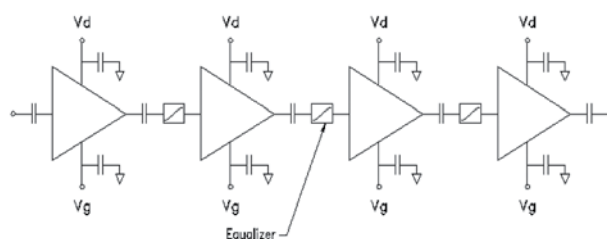
Typical Broadband Module for Fiber Optic SONET
