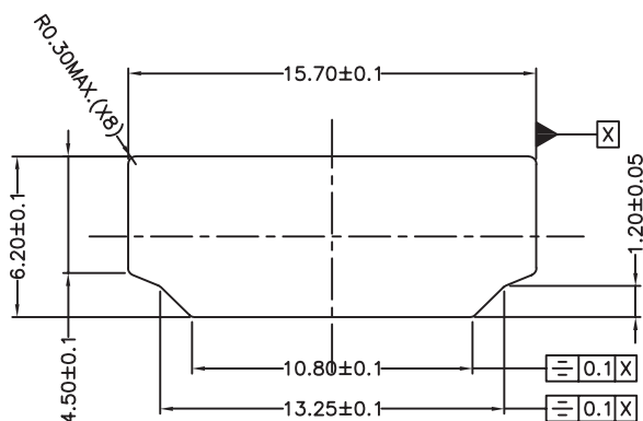
Reference Panel Cut Out Dimension
