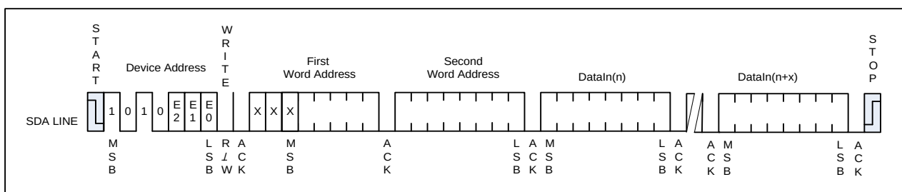
Figure 5-2 Page Write
