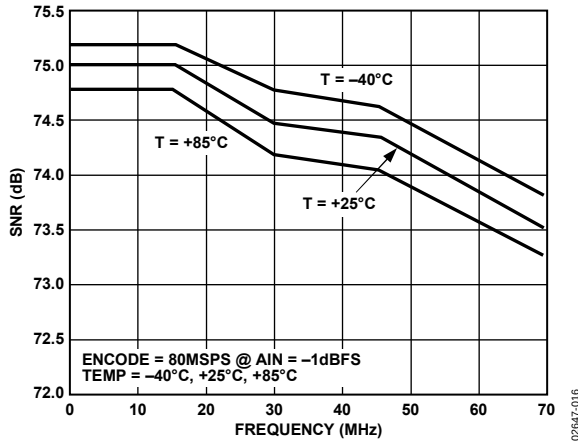
Figure 10. Signal-to-Noise Ratio (SNR) vs. Frequency
