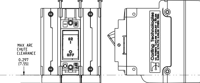
3-POLE (CF3,CG3,C13,C23) w/ ARC CHUTE BARRIER
