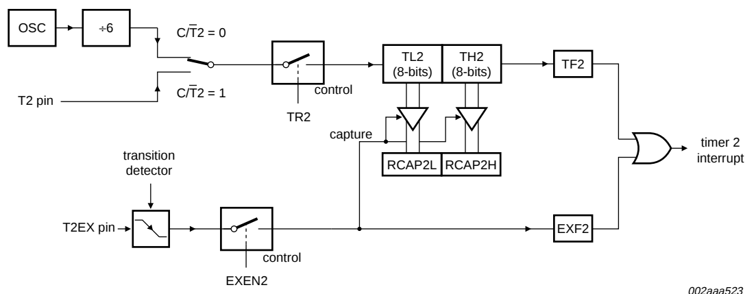
Fig 14. Timer 2 in Capture mode
