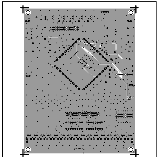
ADES1754 EV Kit PCB Layout—GND 3
