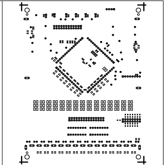
ADES1754 EV Kit Component Placement Guide—Bottom Silkscreen
