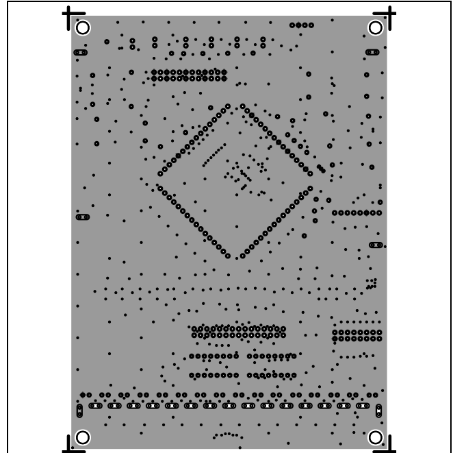
ADES1754 EV Kit PCB Layout—Layer 2
