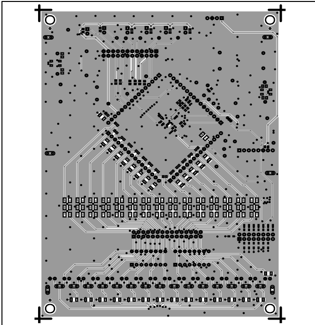
ADES1754 EV Kit PCB Layout—Bottom
