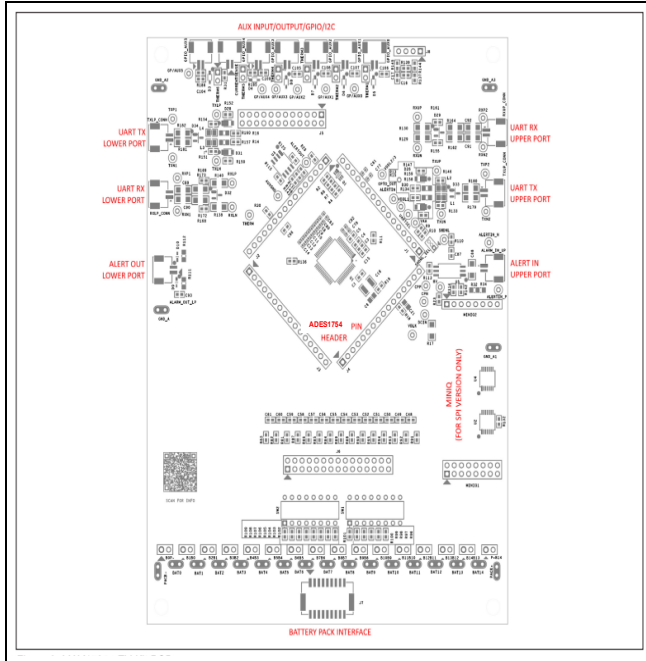
ADES1754 EV Kit Component Placement Guide—Top Silkscreen
