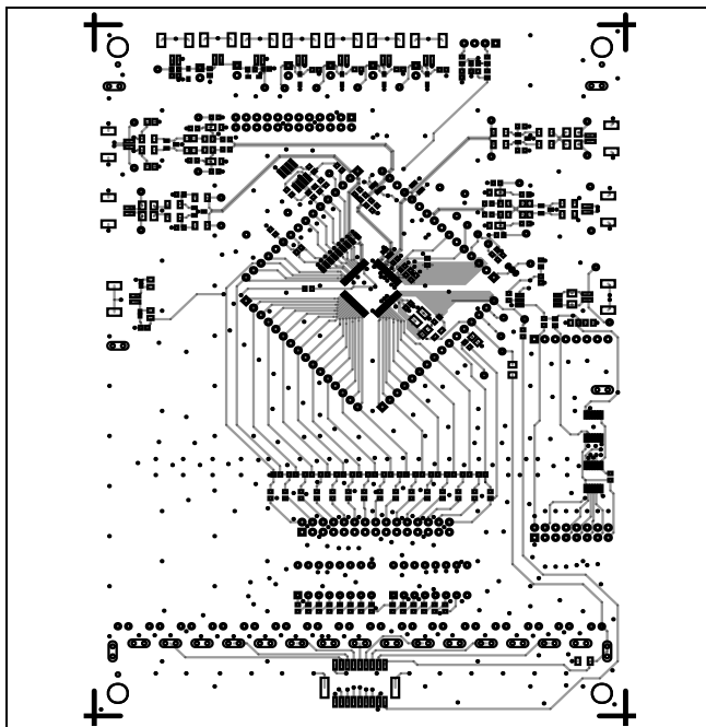
ADES1754 EV Kit PCB Layout—Top
