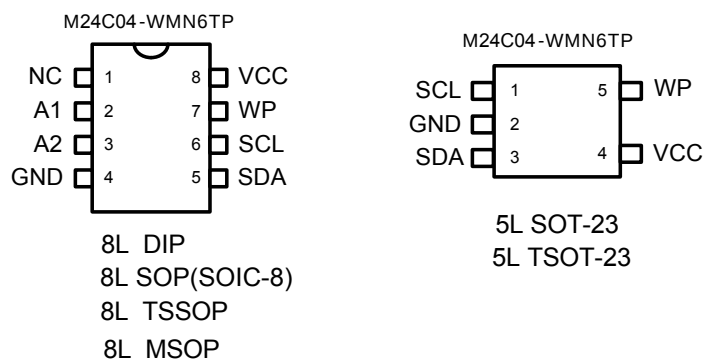
Figure 1: Package types
