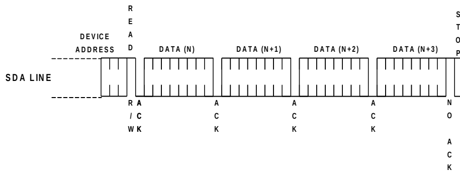
Figure 8: Sequential Read
