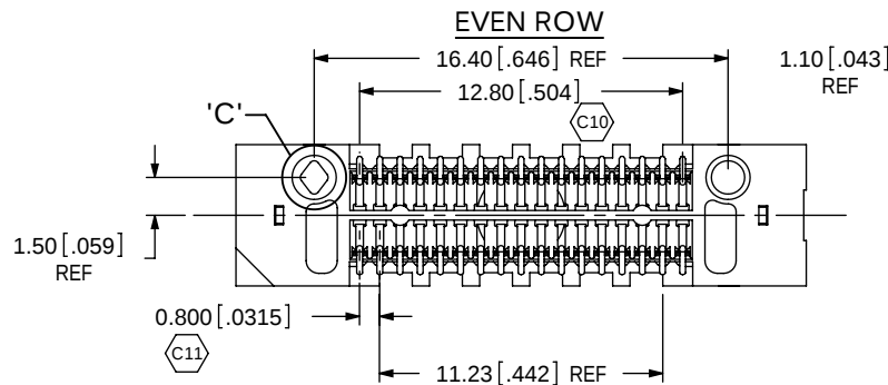
DETAIL 'C' SCALE 6 : 1
