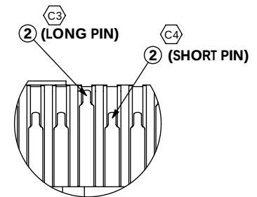
DETAIL 'D' SCALE 6 : 1 DP SIDE
